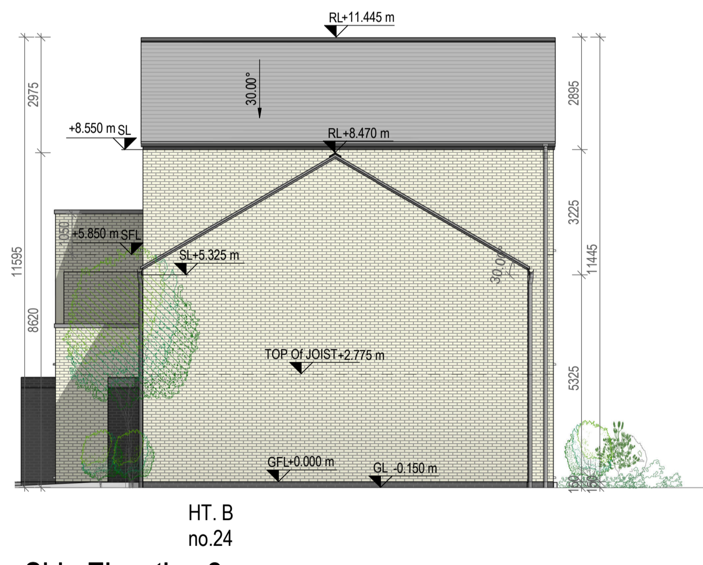
4 Side Elevation 2 1 : 100
